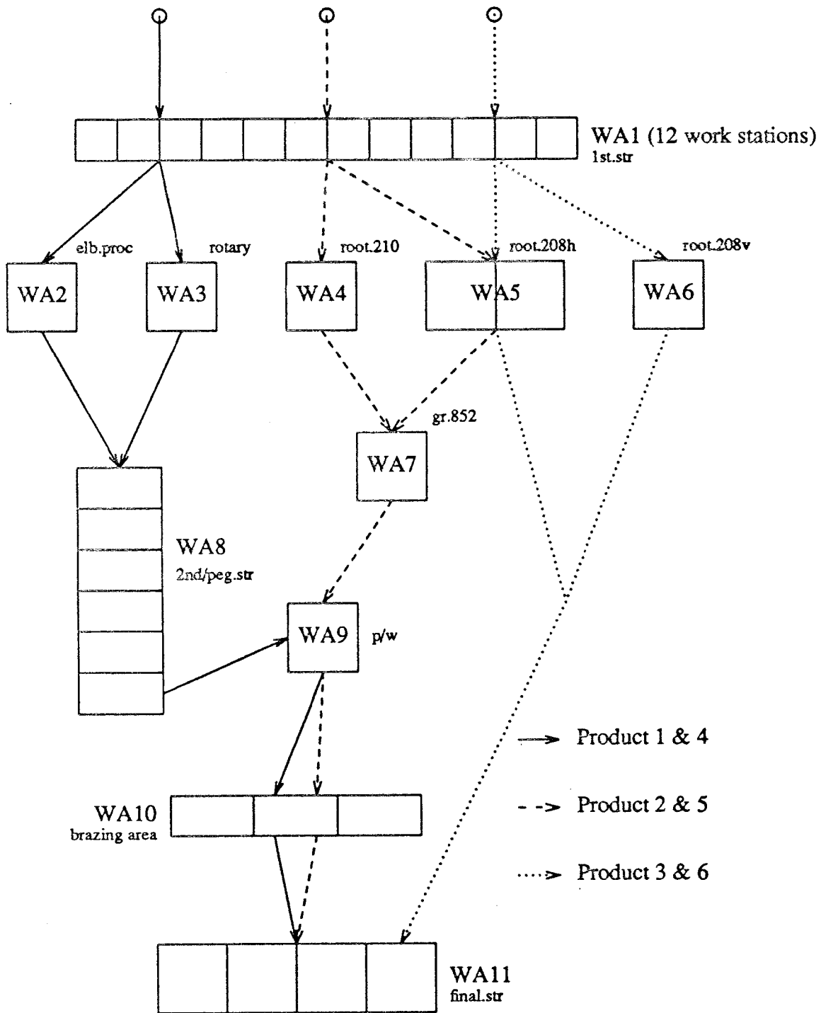
Figure 2: Jobshop Model
